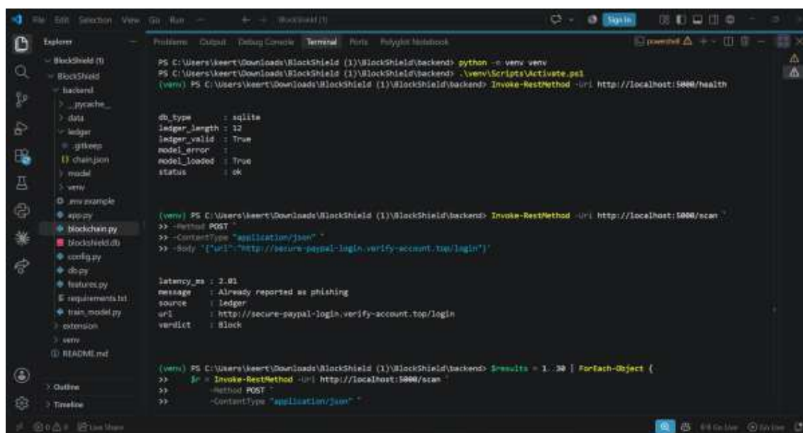
Figure 4.6 Terminal output of /health and /scan requests
