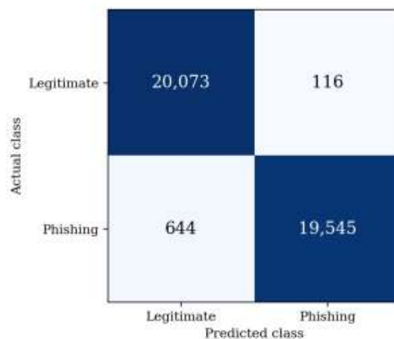
Figure 4.2 Confusion matrix on the test set
