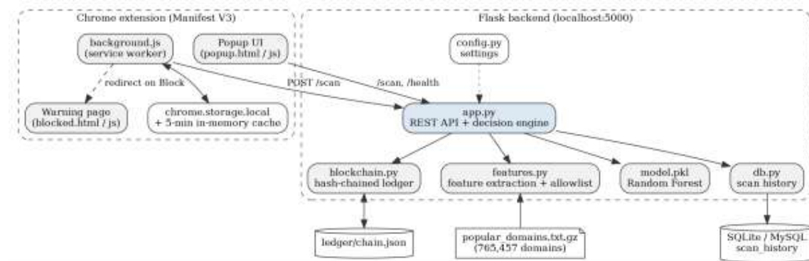
Figure 3.1 System architecture of Block Shield
