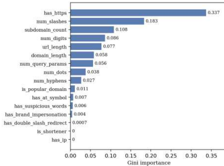
Figure 4.3 Feature importance of the Random Forest
