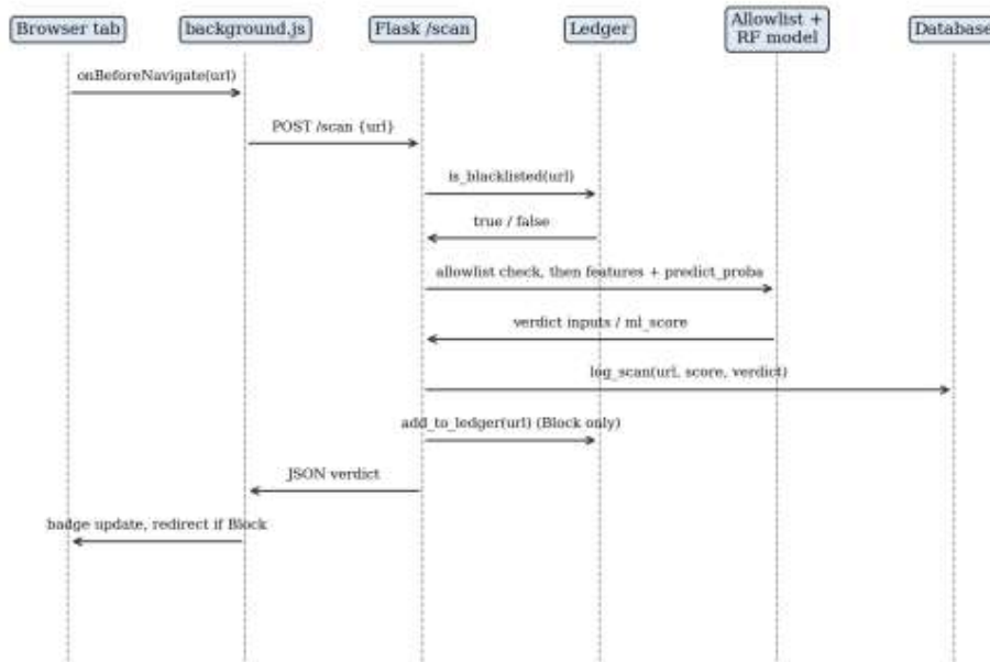
Figure 3.5 Sequence diagram for a navigation event
