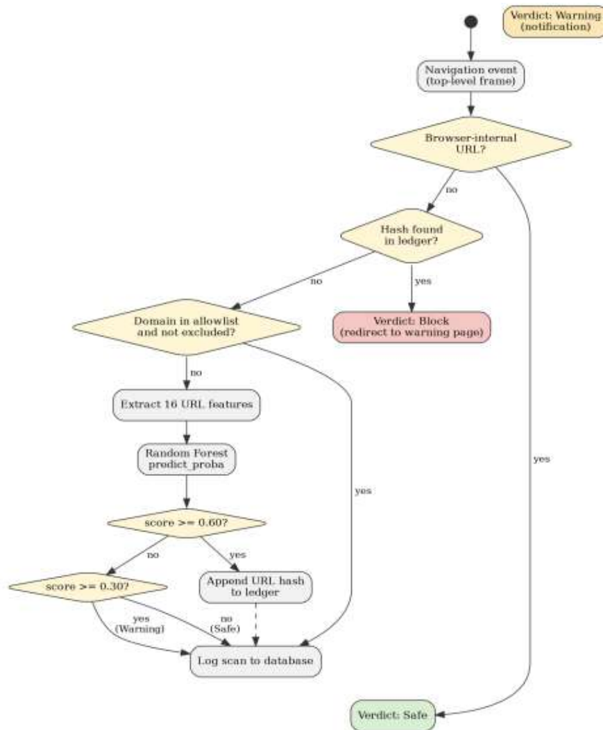
Figure 3.4 Activity diagram of a single scan
