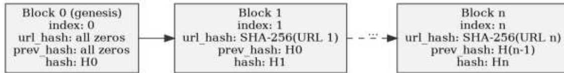
Figure 3.2 Structure of the hash-chained ledger
