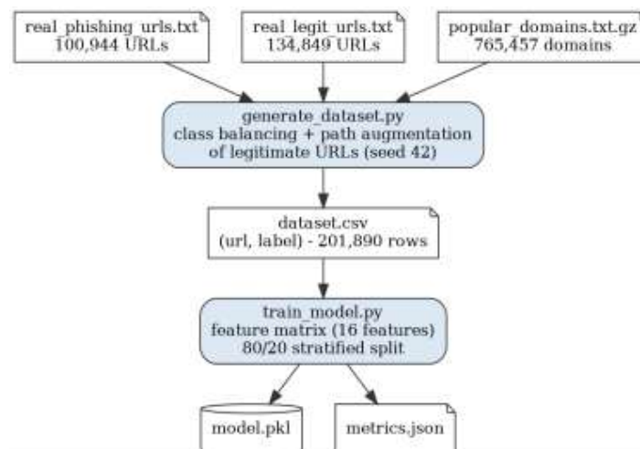
Figure 4.1 Dataset preparation and training flow
